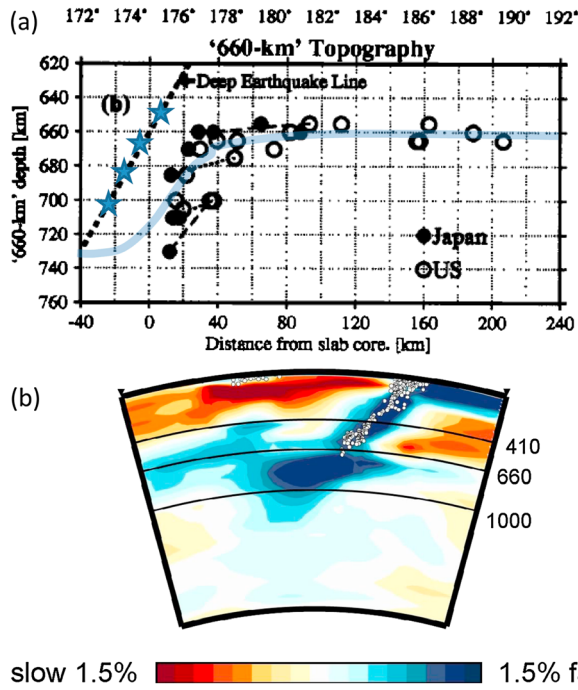
Figure 20. (a) Seismologically-determined phase boundary depths (closed and open circles) of the postspinal transition across the Tonga-Kermadec arc [Niu and Kawakatsu, 1995]. Dotted line represents the deep seismic zone, which is assumed to be the slab core. The pointwise estimated phase boundary depths are smoothly connected by the present authors. Deepest shocks (marked by stars) are schematically added by the present authors, and extend to depths of 700 km. (b) Tomographic cross section across the Kermadec arc (the same as cross section F in Figure 10).
