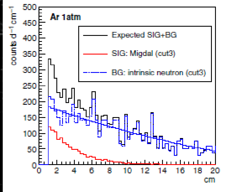
Distance between clusters
