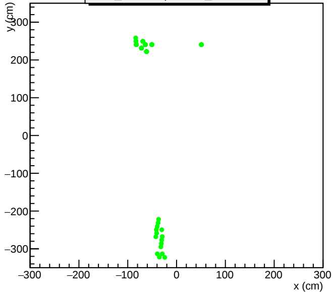
2017 Feb.17 cosmic run_ID=716, event_ID=4221
