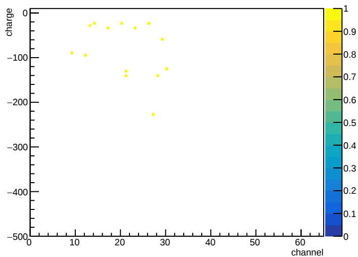
20170217 cosmic aux BF0, layer0 phi
