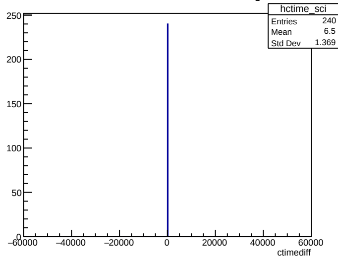
20170217 cosmic aux BF4 scitime-trigtime
