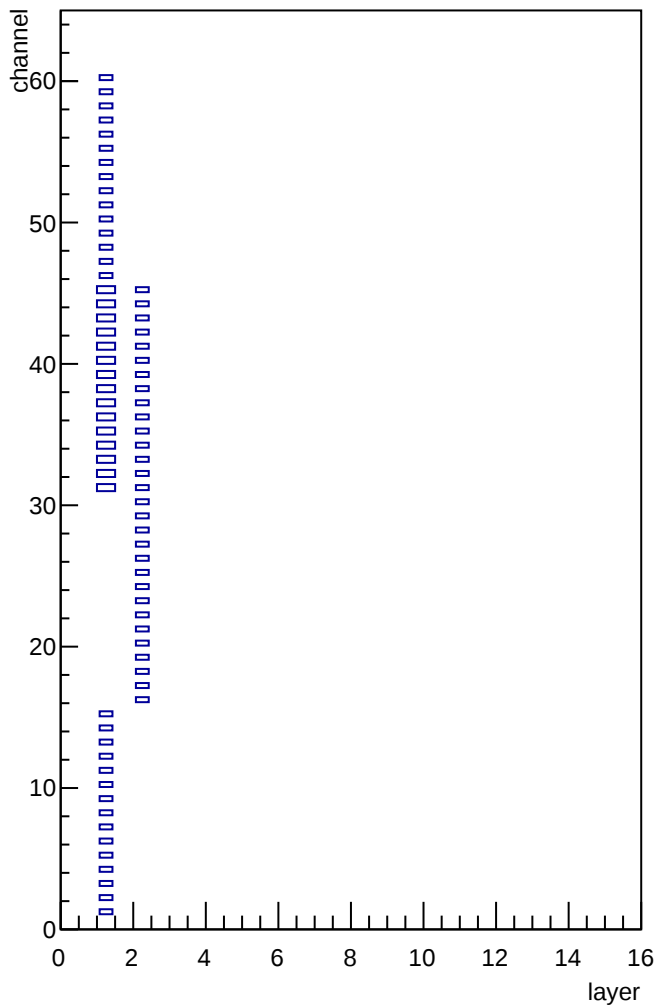
20170217 cosmic aux BF3 z
