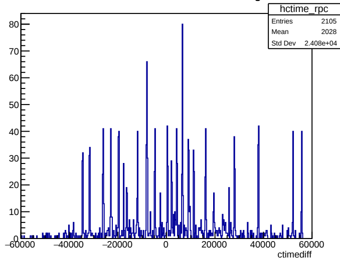
20170217 cosmic aux BF6 scitime-trigtime
