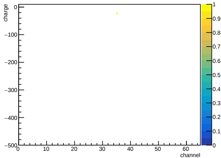
20170217 cosmic aux BB3, layer0 phi
