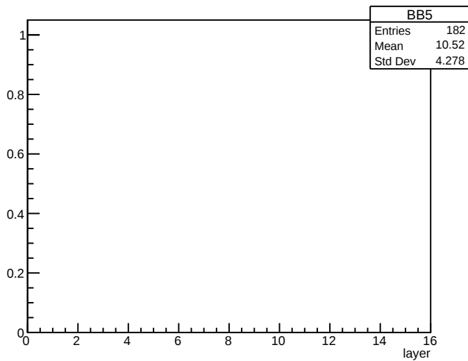
20170217 cosmic aux BB5
