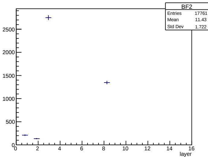
20170217 cosmic aux BF2
