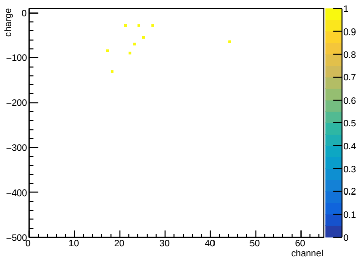
20170217 cosmic aux BF4, layer0 z
