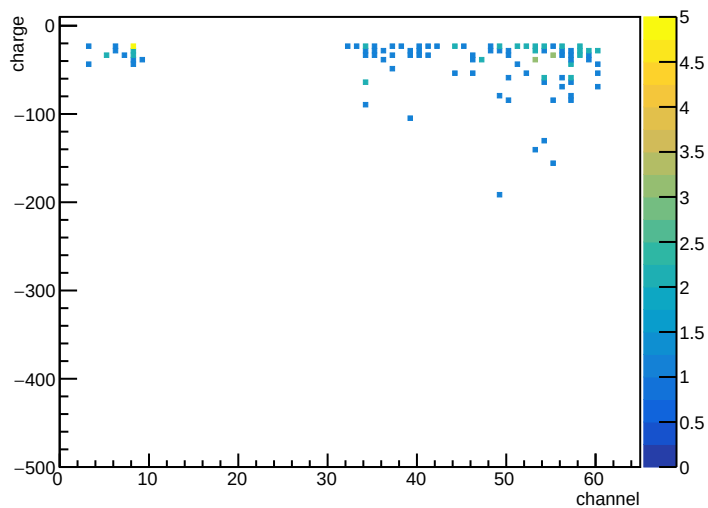
20170208 cosmic layer[2] z BF2
