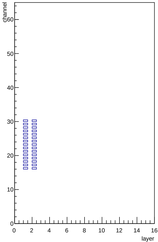
20170208 cosmic z-measuring BF7
