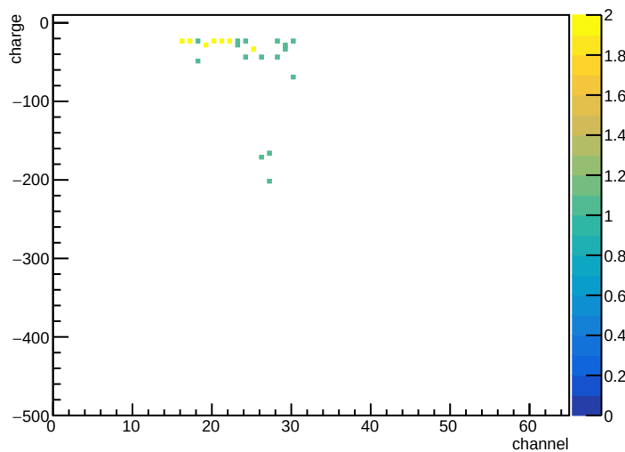
20170208 cosmic layer[1] z BF7
