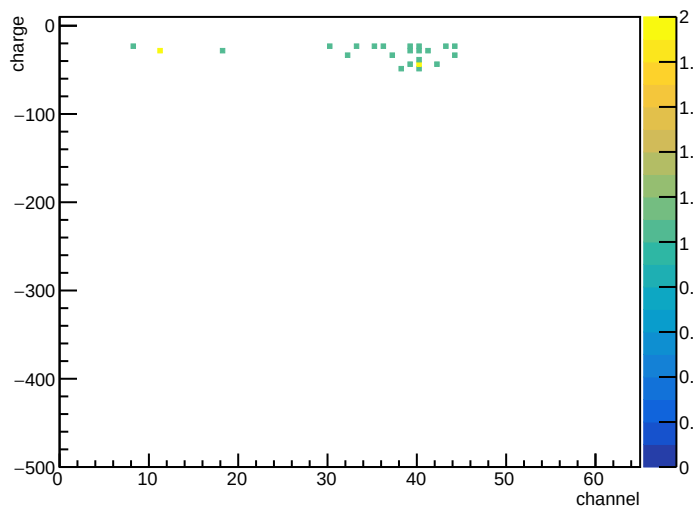
20170208 cosmic layer[2] phi BF2
