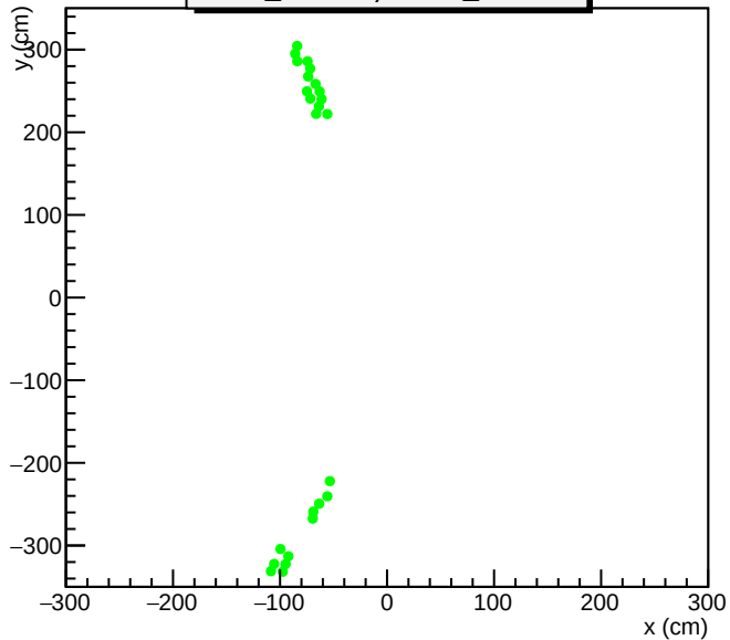
2017 Feb.08 cosmic run_ID=139, event_ID=63
