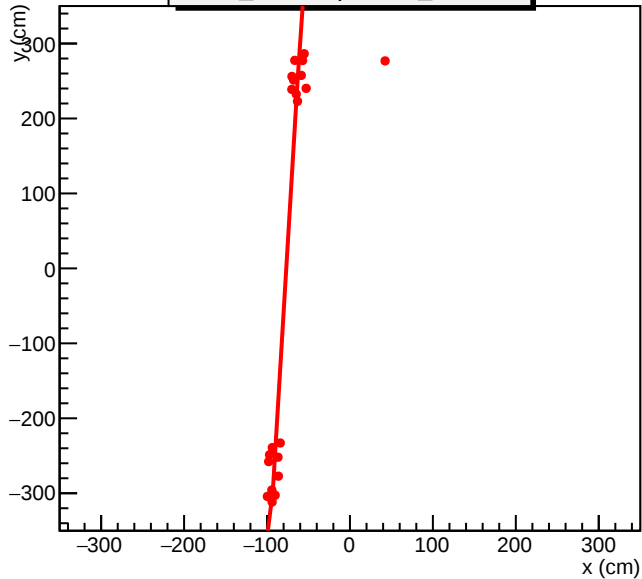
2017 Feb.08 cosmic run_ID=176, event_ID=37
