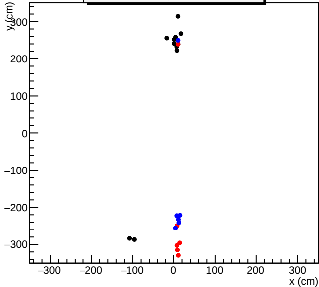
2017 Feb.08 cosmic run_ID=181, event_ID=22
