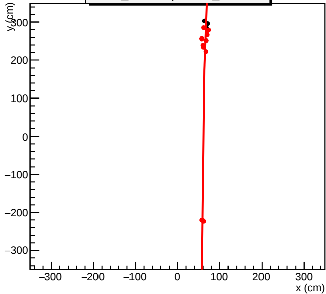
2017 Feb.08 cosmic run_ID=149, event_ID=99
