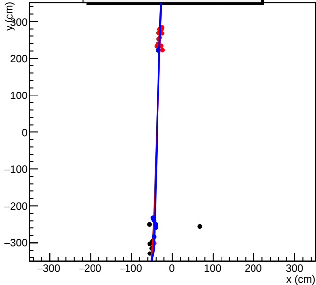
2017 Feb.08 cosmic run_ID=174, event_ID=59
