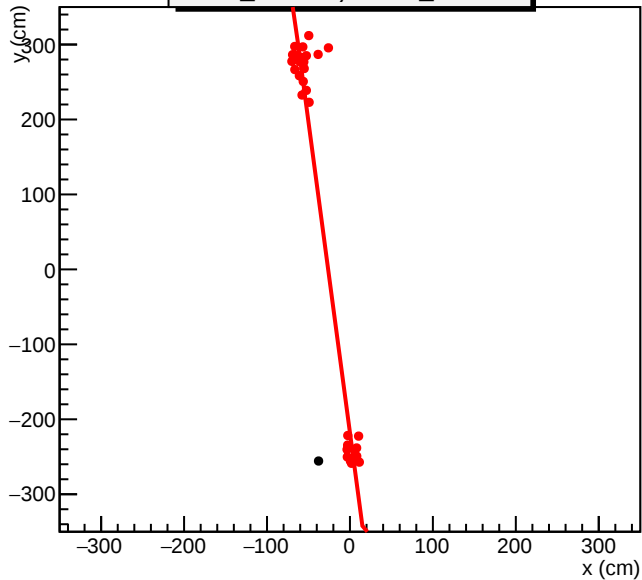
2017 Feb.08 cosmic run_ID=172, event_ID=21
