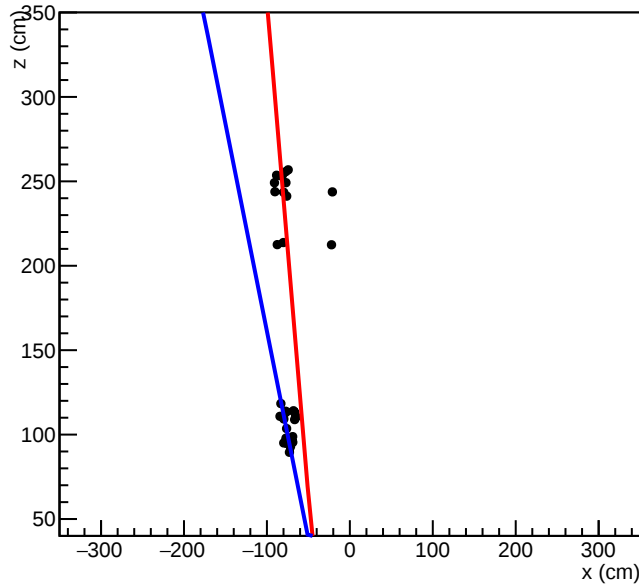
2017 Feb.08 cosmic
