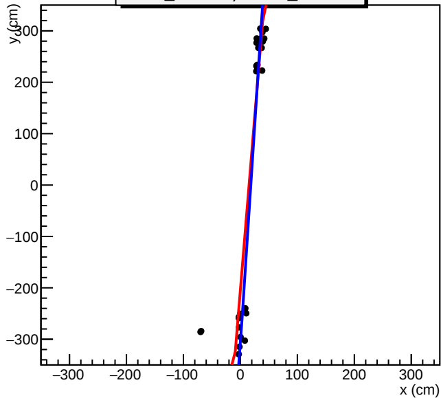
2017 Feb.08 cosmic run_ID=179, event_ID=47
