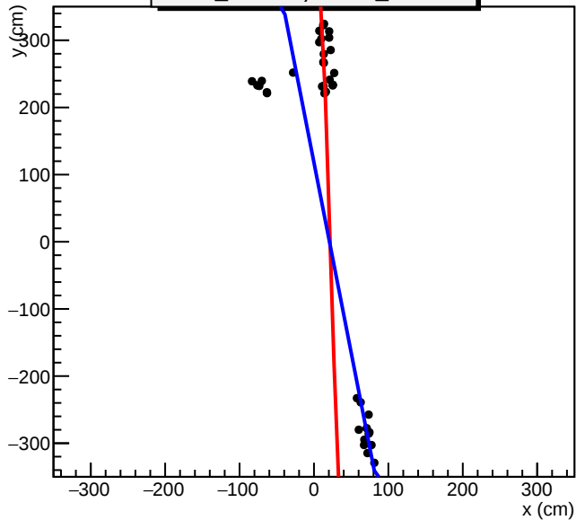
2017 Feb.08 cosmic run_ID=173, event_ID=18
