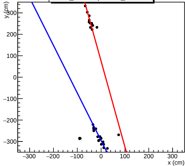
2017 Feb.08 cosmic run_ID=163, event_ID=46
