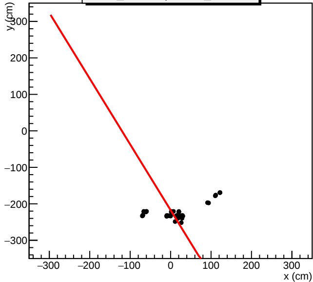
2017 Feb.08 cosmic run_ID=146, event_ID=36
