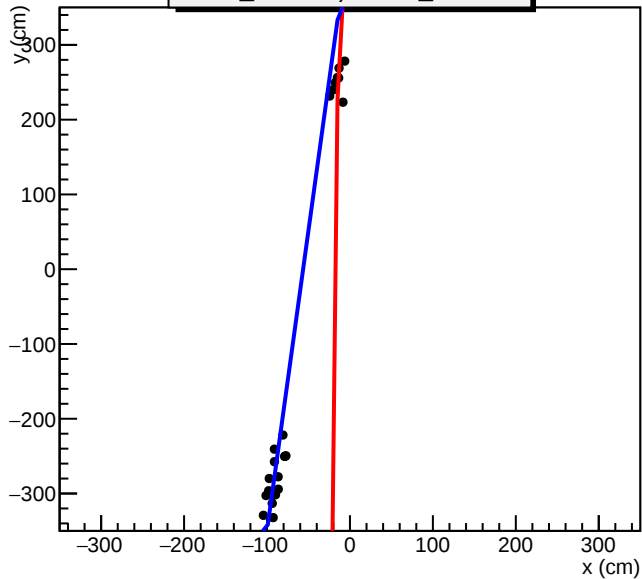
2017 Feb.08 cosmic run_ID=158, event_ID=37
