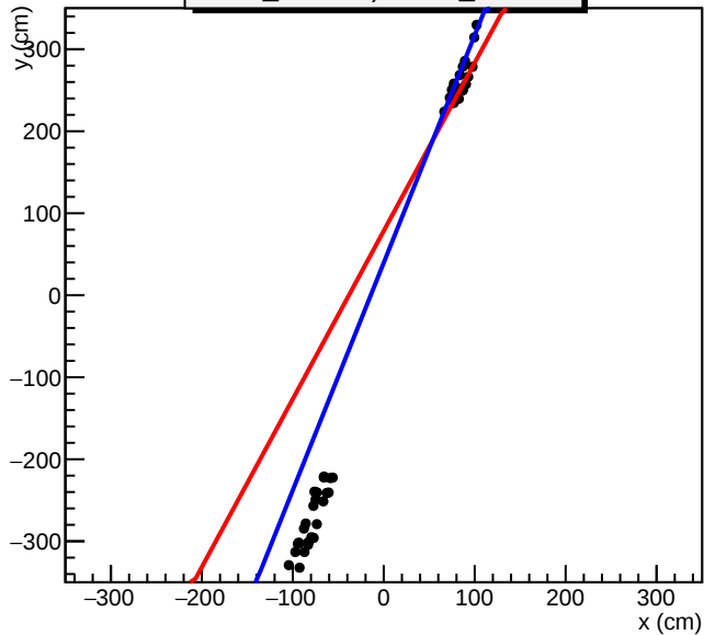
2017 Feb.08 cosmic run_ID=169, event_ID=24
