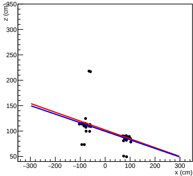
2017 Feb.08 cosmic
