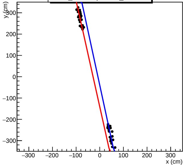
2017 Feb.08 cosmic run_ID=182, event_ID=80
