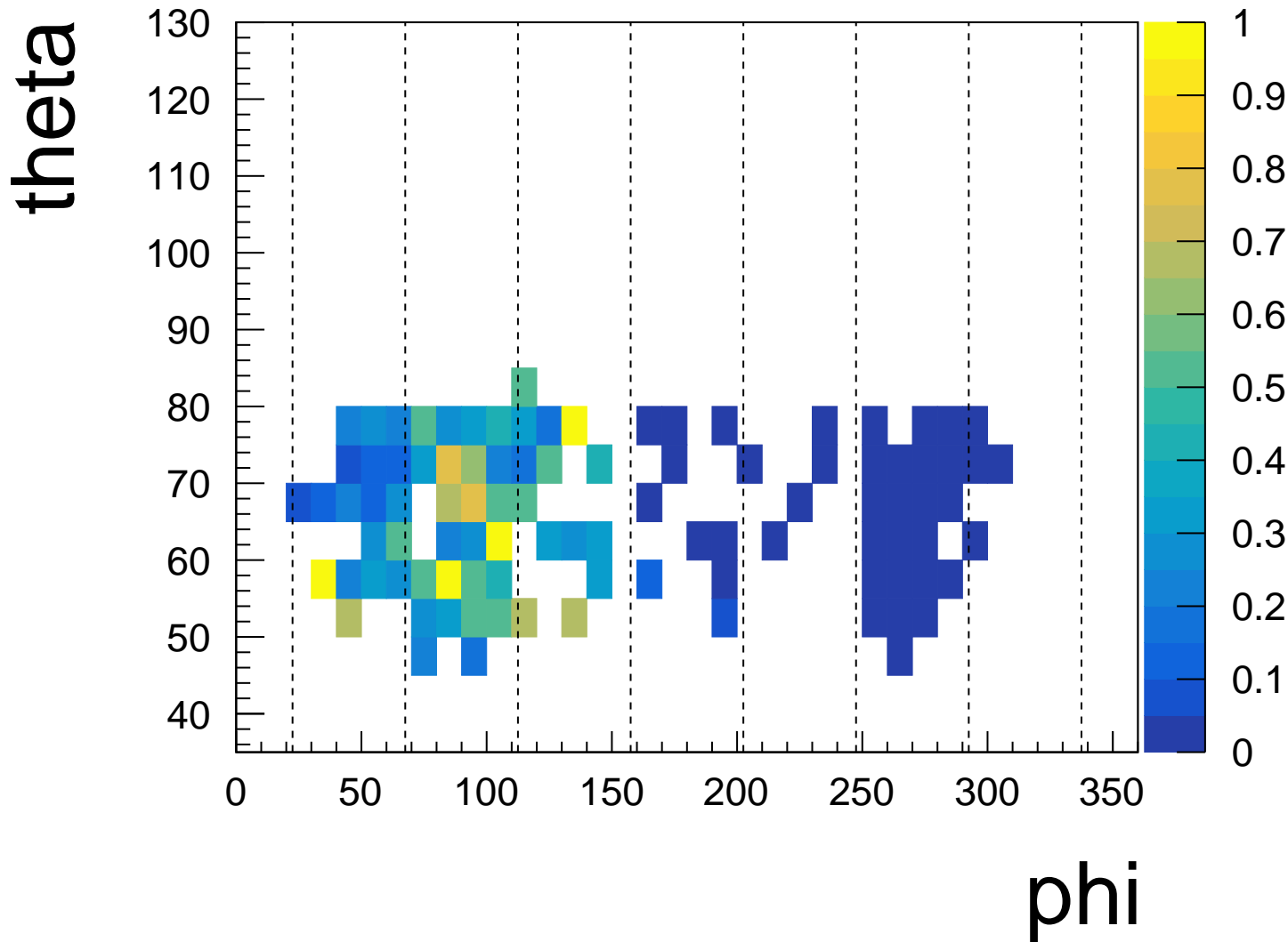
Efficiency for BKLM layer 8
