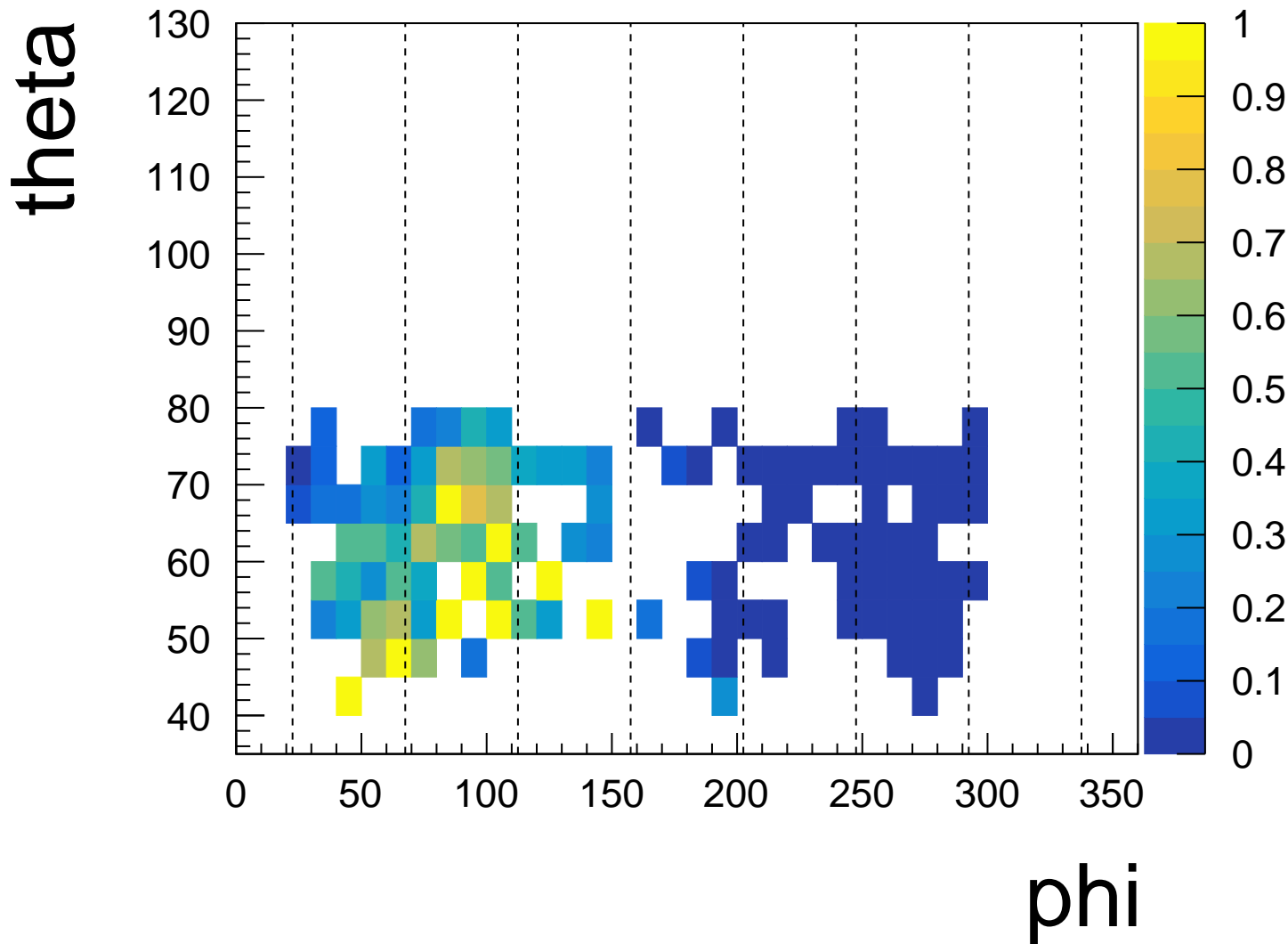
Efficiency for BKLM layer 3
